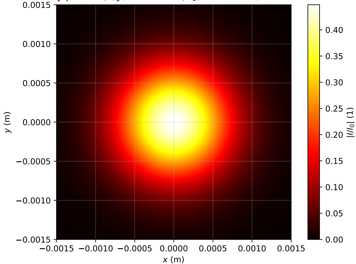
Intensity profile I(x, y, z = 2.388m)/I_0 , P_{in}=0.1P_{cr} , artificial time
